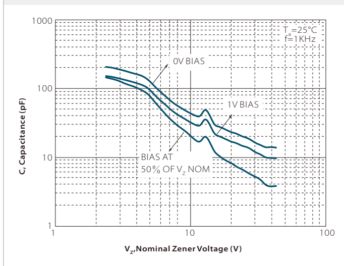
Typical Capacitance
